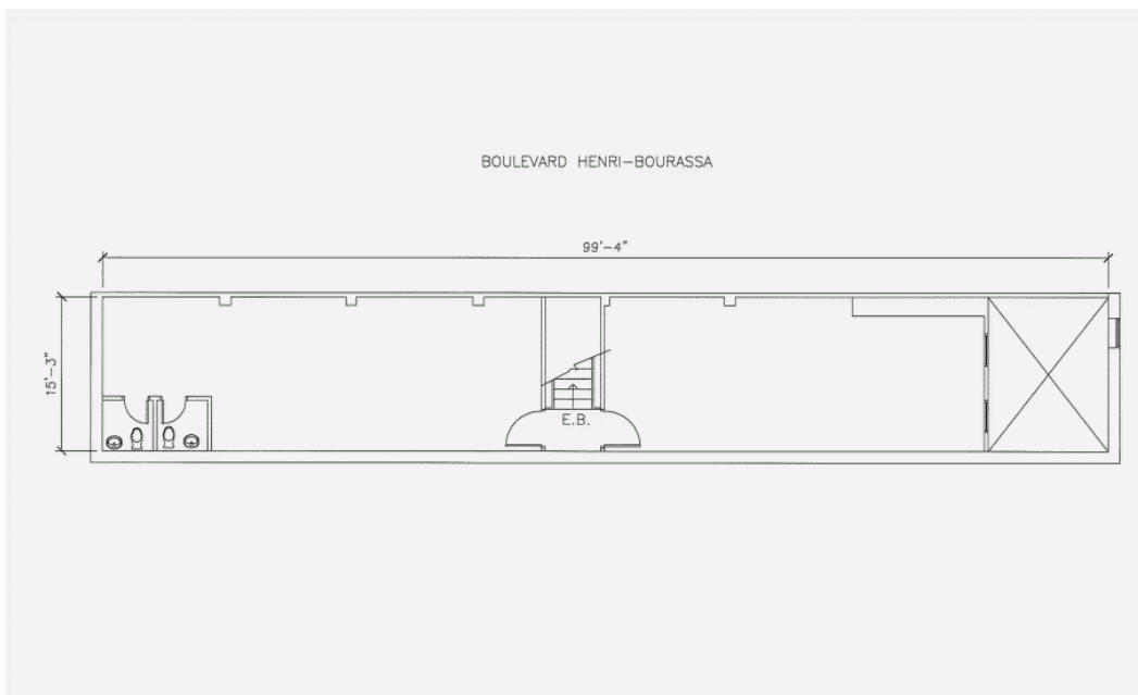
Layout plan - floor
